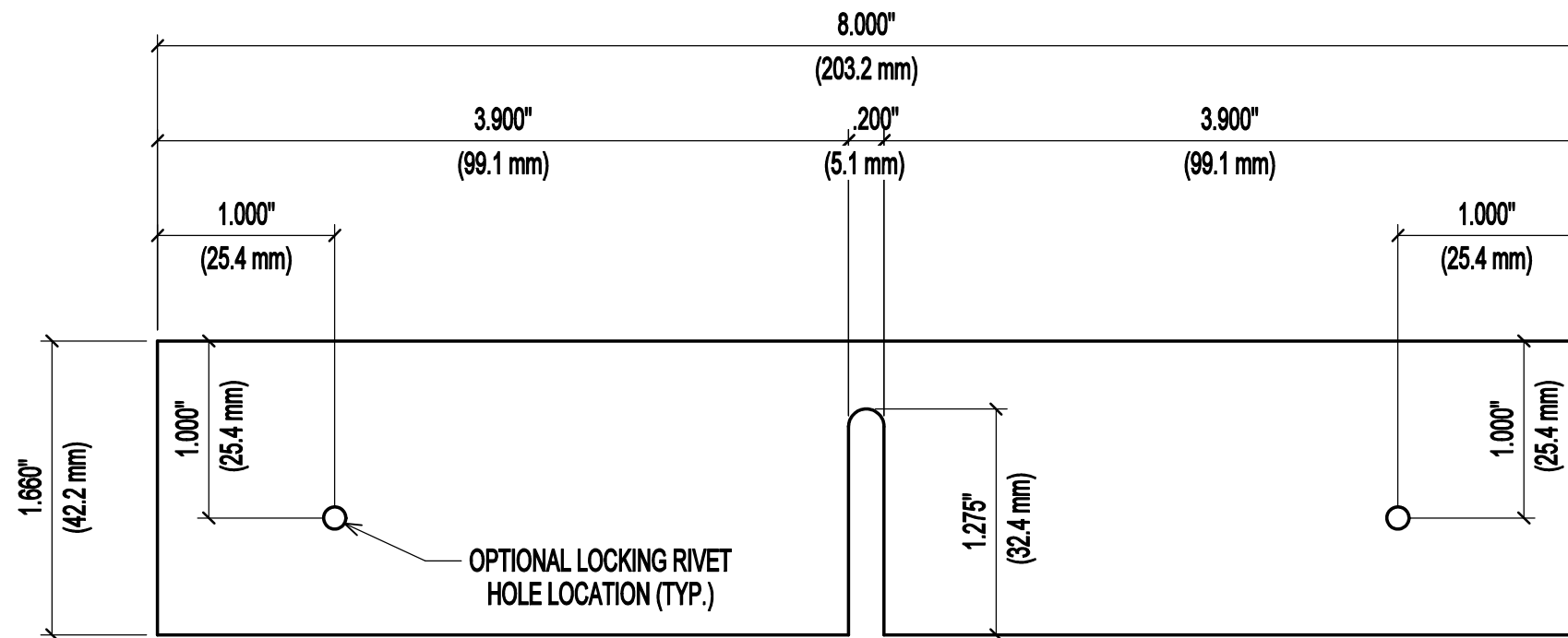
SIDE VIEW - TR35 - OFFSET CLAMP #TR-5030 FULL SCALE
