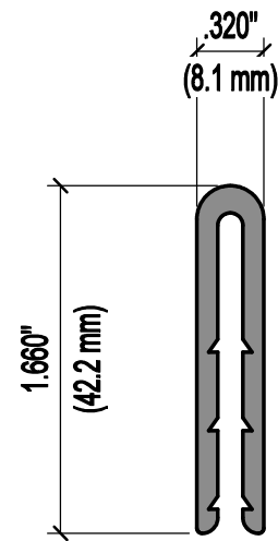
FRONT VIEW - TR35 - OFFSET CLAMP #TR-5030 FULL SCALE
