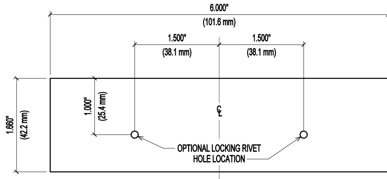
SIDE VIEW - TR35 - SPLICE CLAMP #TR-5020 FULL SCALE
