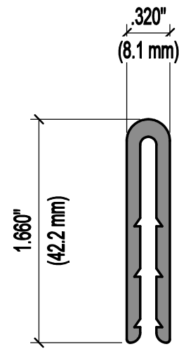
FRONT VIEW - TR35 - SPLICE CLAMP #TR-5020 FULL SCALE
