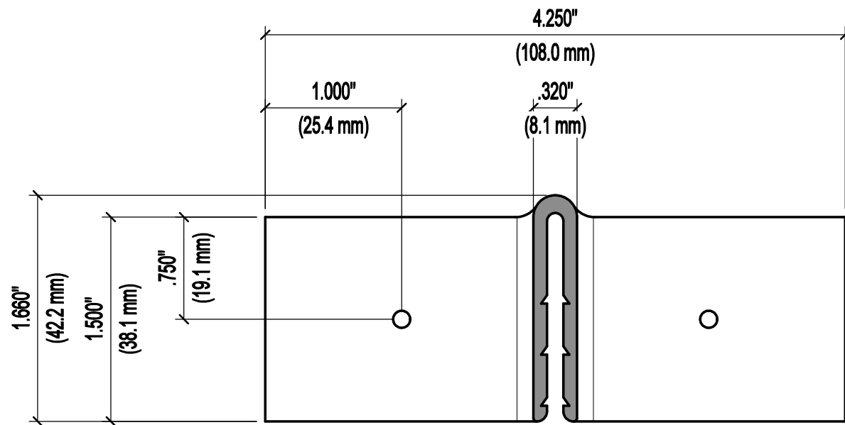
FRONT VIEW - TR35 - T CLAMP #TR-5010 FULL SCALE
