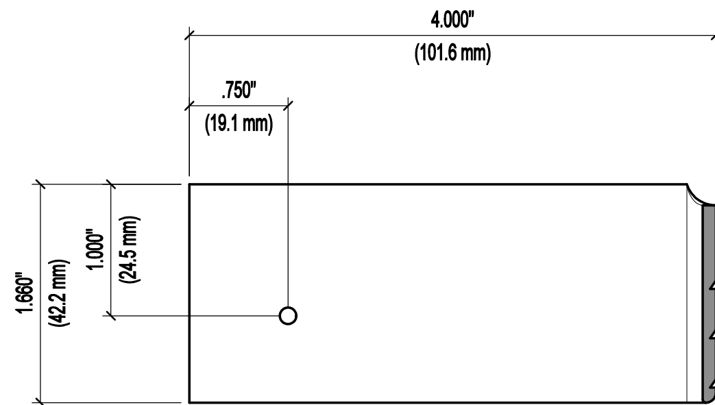
SIDE VIEW - TR35 - T CLAMP #TR-5010 FULL SCALE
