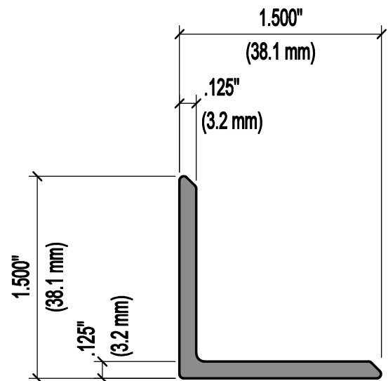
WALL RAIL SECTION - #TR-5060 FULL SCALE
