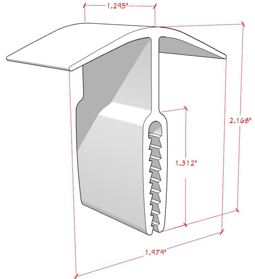
SIDE VIEW - TR35 - HIGH PANEL CLIP - DOUBLE #TR-5052D FULL SCALE
