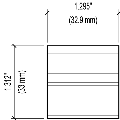
SIDE VIEW - TR35 - MID PANEL CLIP - SINGLE #TR-5051S FULL SCALE
