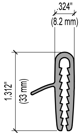
FRONT VIEW - TR35 - MID PANEL CLIP - SINGLE #TR-5051S FULL SCALE
