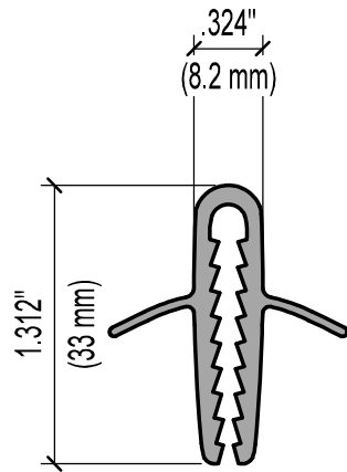
FRONT VIEW - TR35 - MID PANEL CLIP - DOUBLE #TR-5051D FULL SCALE
