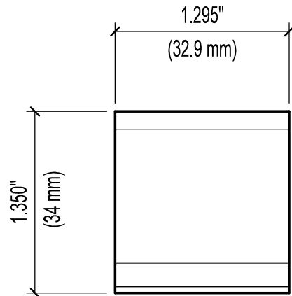
SIDE VIEW - TR35 - LOW PANEL CLIP - SINGLE #TR-5050S FULL SCALE
