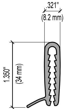
FRONT VIEW - TR35 - LOW PANEL CLIP - SINGLE #TR-5050S FULL SCALE
