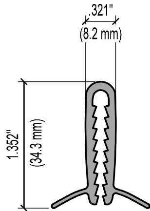
FRONT VIEW - TR35 - LOW PANEL CLIP - DOUBLE #TR-5050D FULL SCALE
