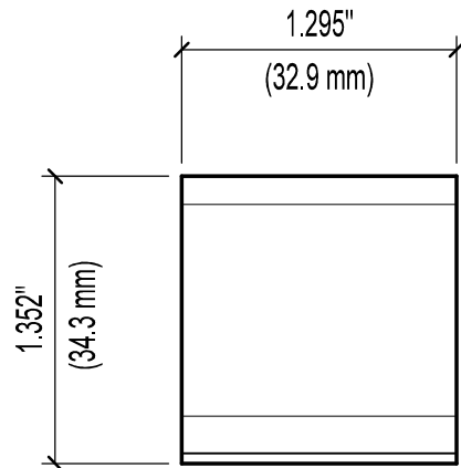
SIDE VIEW - TR35 - LOW PANEL CLIP - DOUBLE #TR-5050D FULL SCALE
