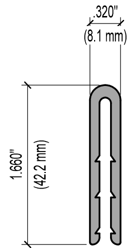
FRONT VIEW - TR35 - MODIFIED CUT INTERLOCK CLAMP #TR-5035 FULL SCALE
