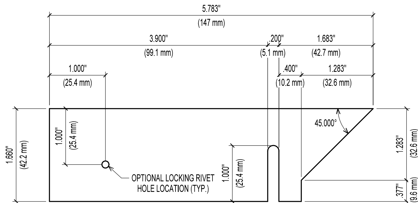
SIDE VIEW - TR35 - MODIFIED CUT INTERLOCK CLAMP #TR-5035 FULL SCALE
