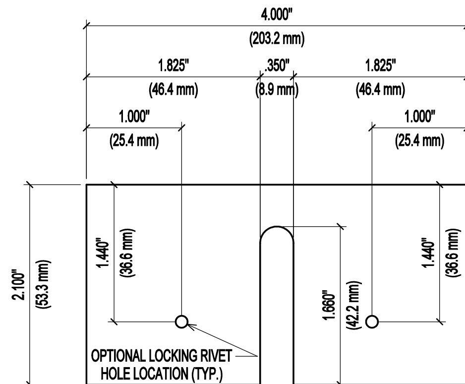
SIDE VIEW - TR35 - OVERLOCK CLAMP #TR-5040 FULL SCALE
