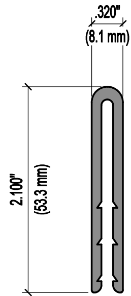
FRONT VIEW - TR35 - OVERLOCK CLAMP #TR-5040 FULL SCALE
