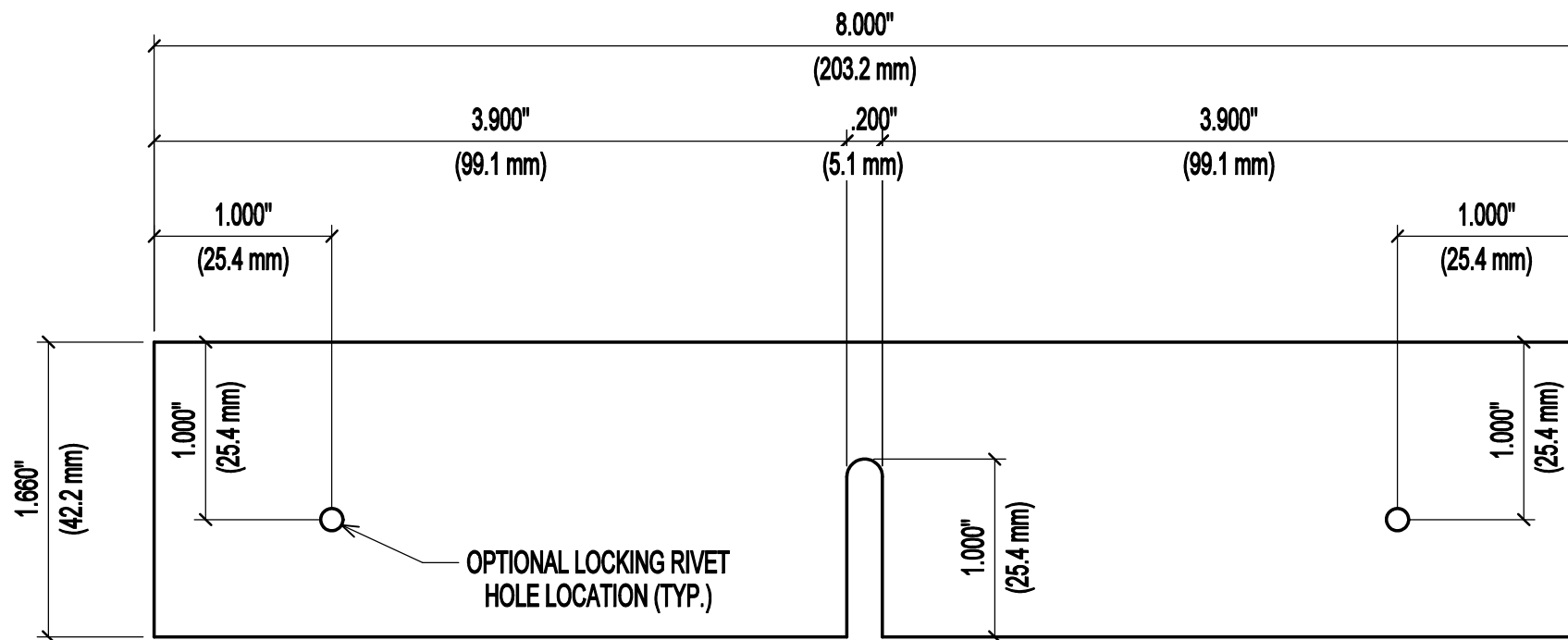
SIDE VIEW - TR35 - INTERLOCK CLAMP #TR-5035 FULL SCALE
