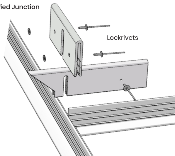
Wallrail
