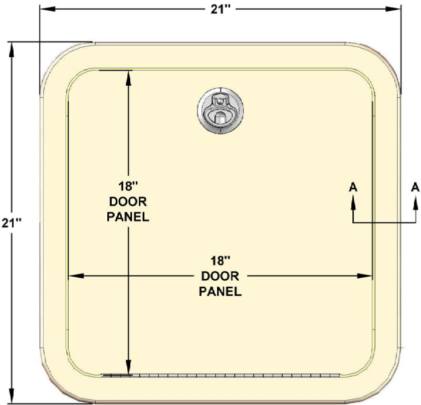
FRONT VIEW #7508 WHITE ACRYLIC
