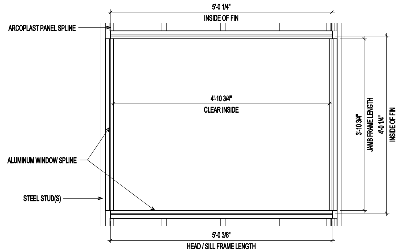
WINDOW ALUMINUM FRAME ELEVATION
