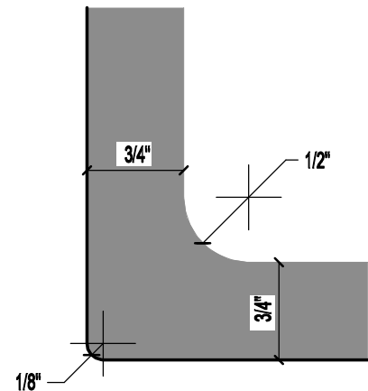
GLASS CORNER DETAIL SCALE: FULL (1:1)
