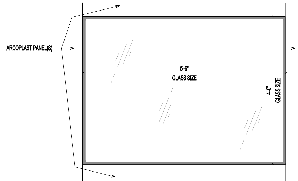
WINDOW ELEVATION SCALE: 3/4" = 1'-0" (1:16)
