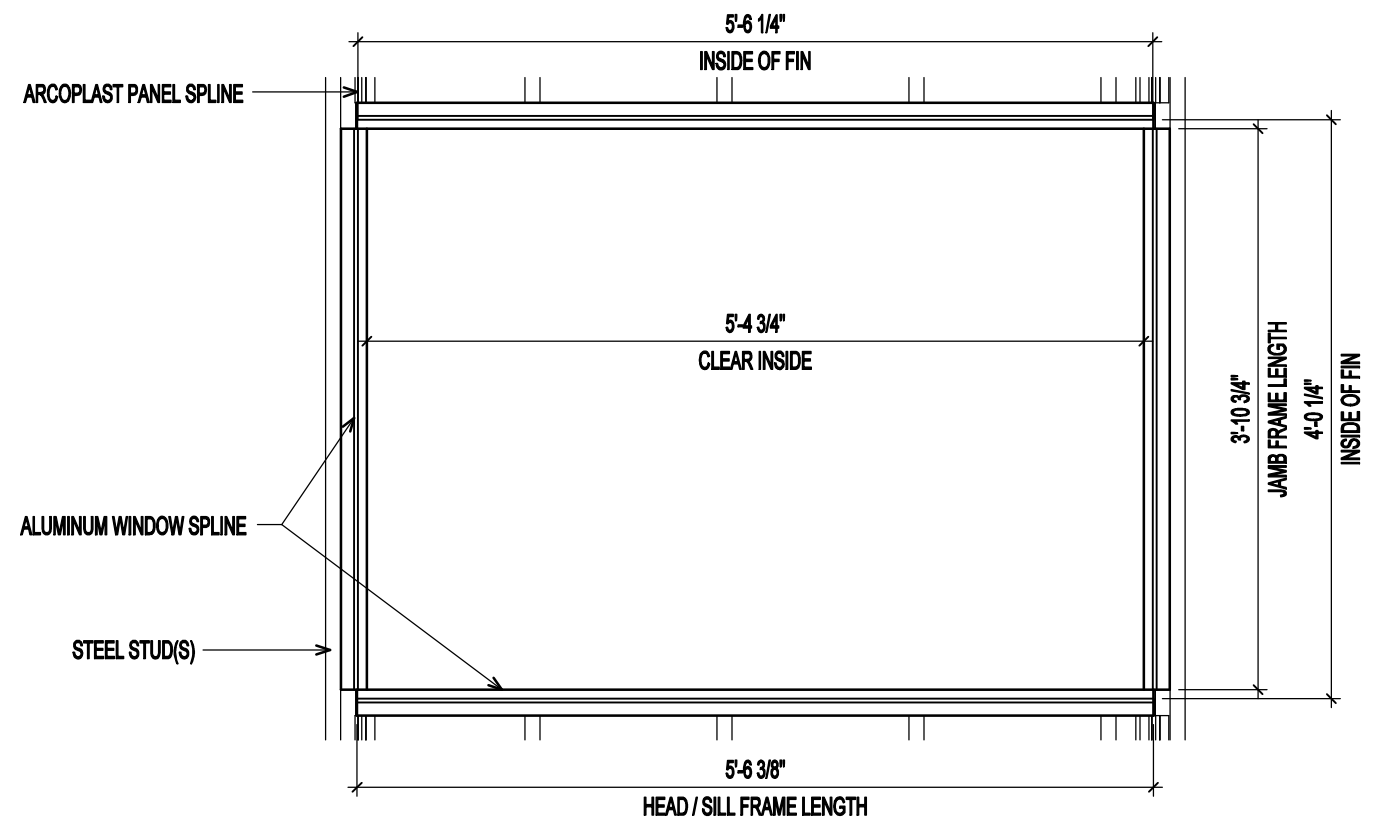
WINDOW ALUMINUM FRAME ELEVATION SCALE: 3/4" = 1'-0" (1:16)
