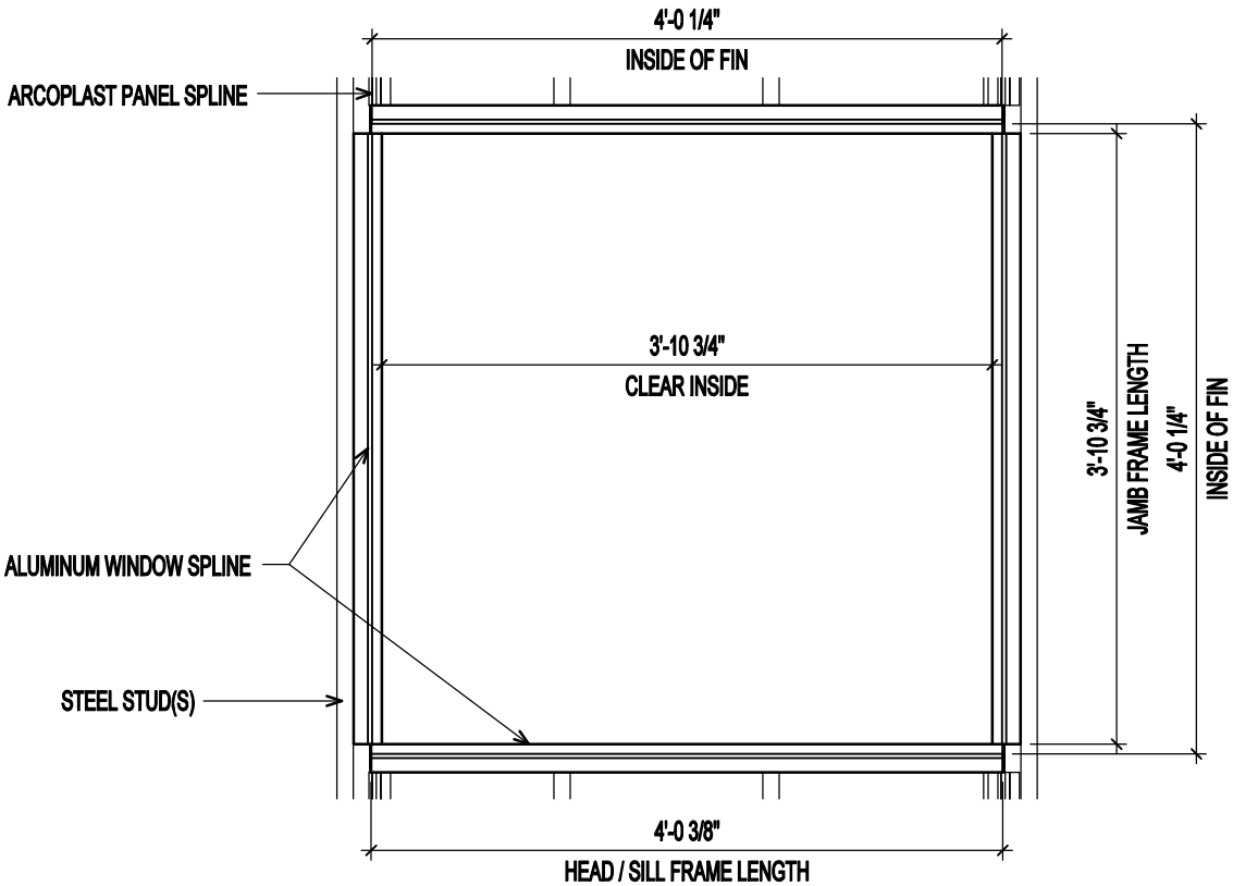
WINDOW ALUMINUM FRAME ELEVATION
