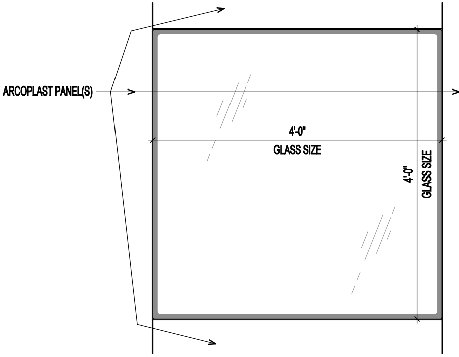
WINDOW ELEVATION
