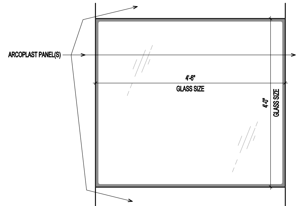
WINDOW ELEVATION
