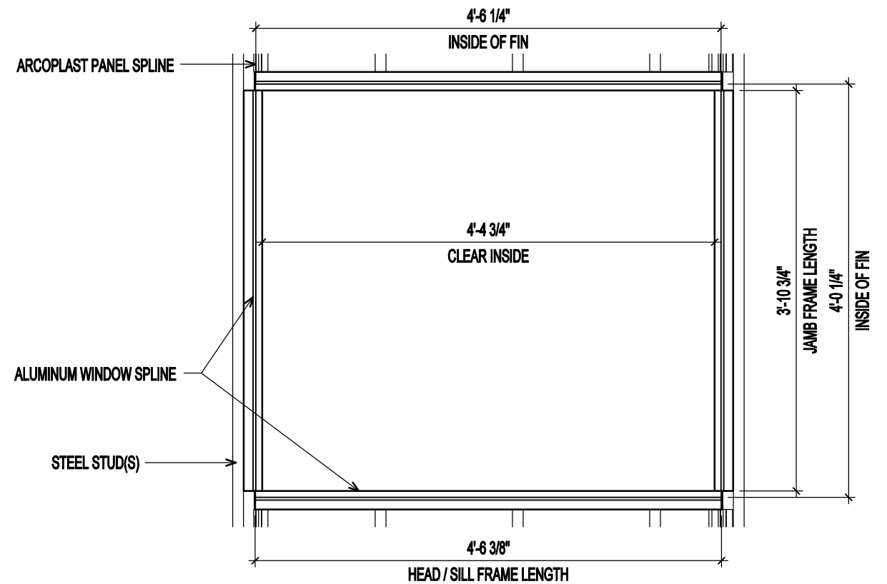
WINDOW ALUMINUM FRAME ELEVATION
