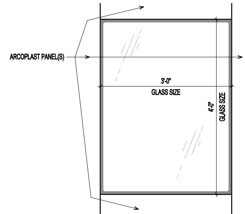
WINDOW ELEVATION
