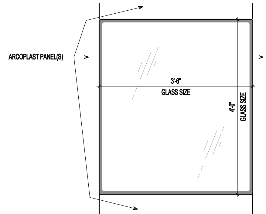
WINDOW ELEVATION
