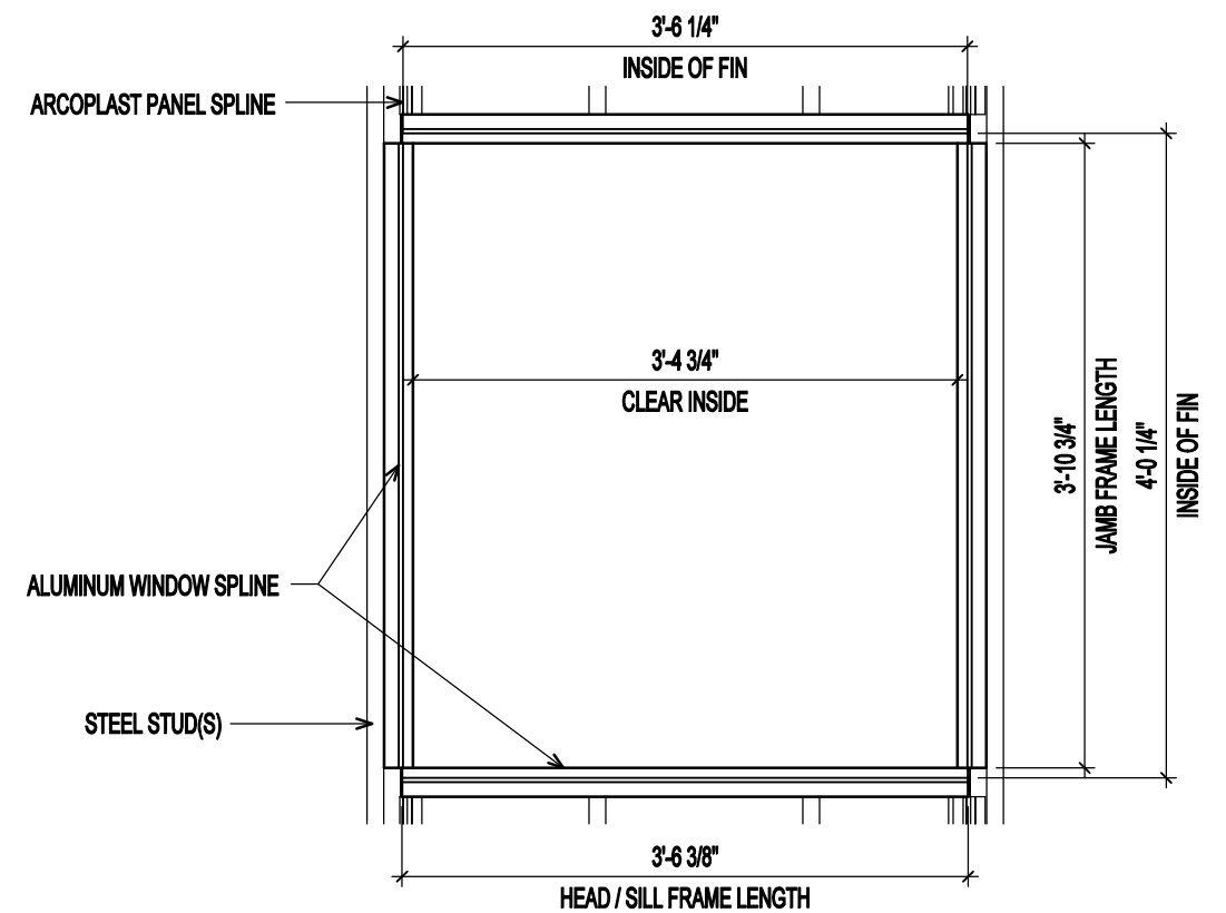
WINDOW ALUMINUM FRAME ELEVATION
