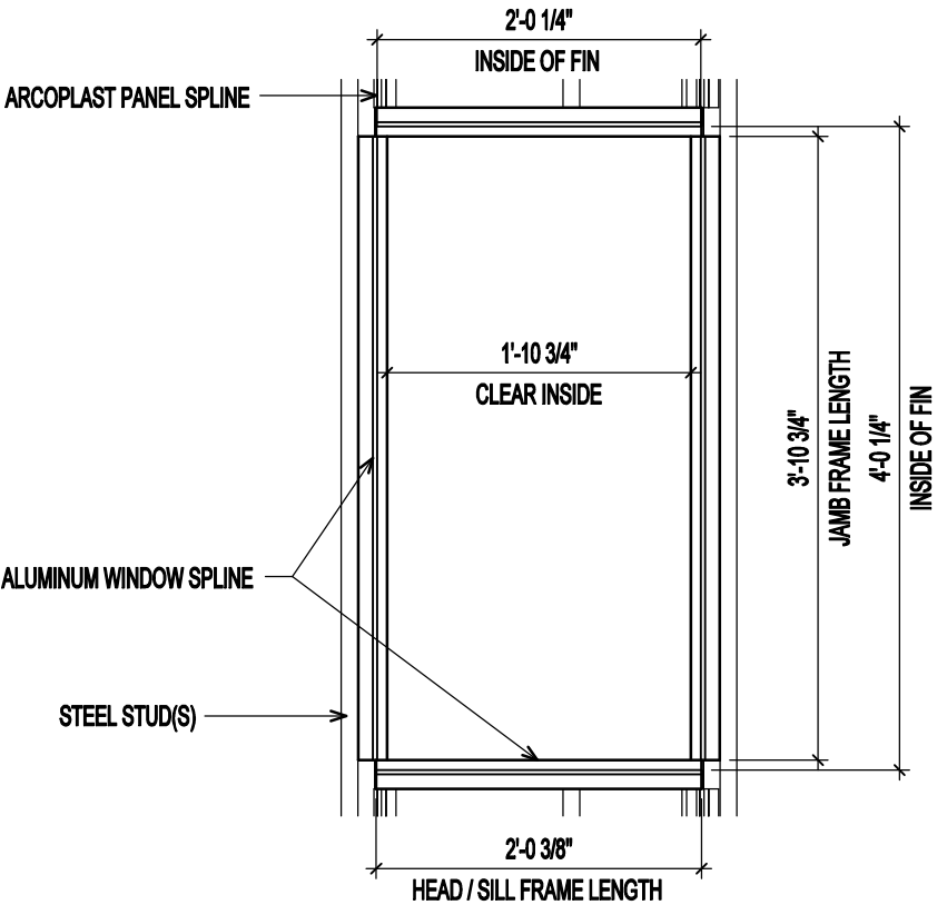
WINDOW ALUMINUM FRAME ELEVATION
