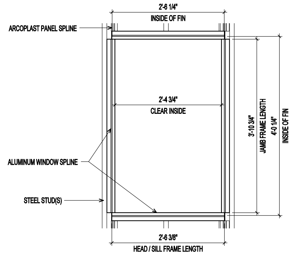
WINDOW ALUMINUM FRAME ELEVATION
