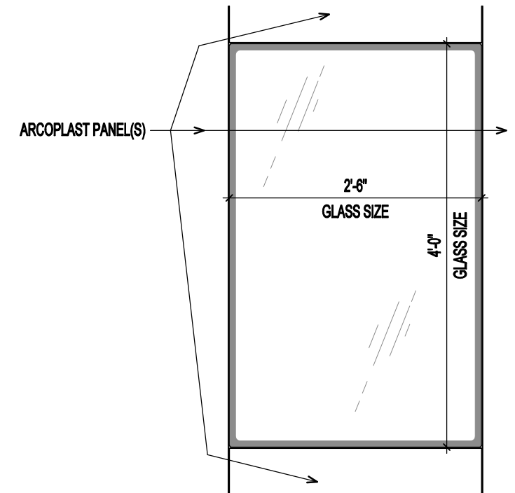
WINDOW ELEVATION
