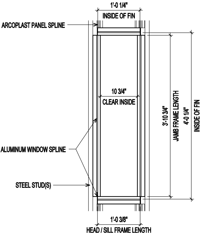
WINDOW ALUMINUM FRAME ELEVATION
