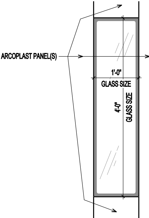
WINDOW ELEVATION
