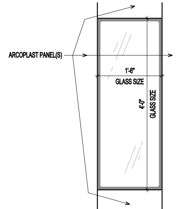
WINDOW ELEVATION SCALE: 3/4" = 1'-0" (1:16)
