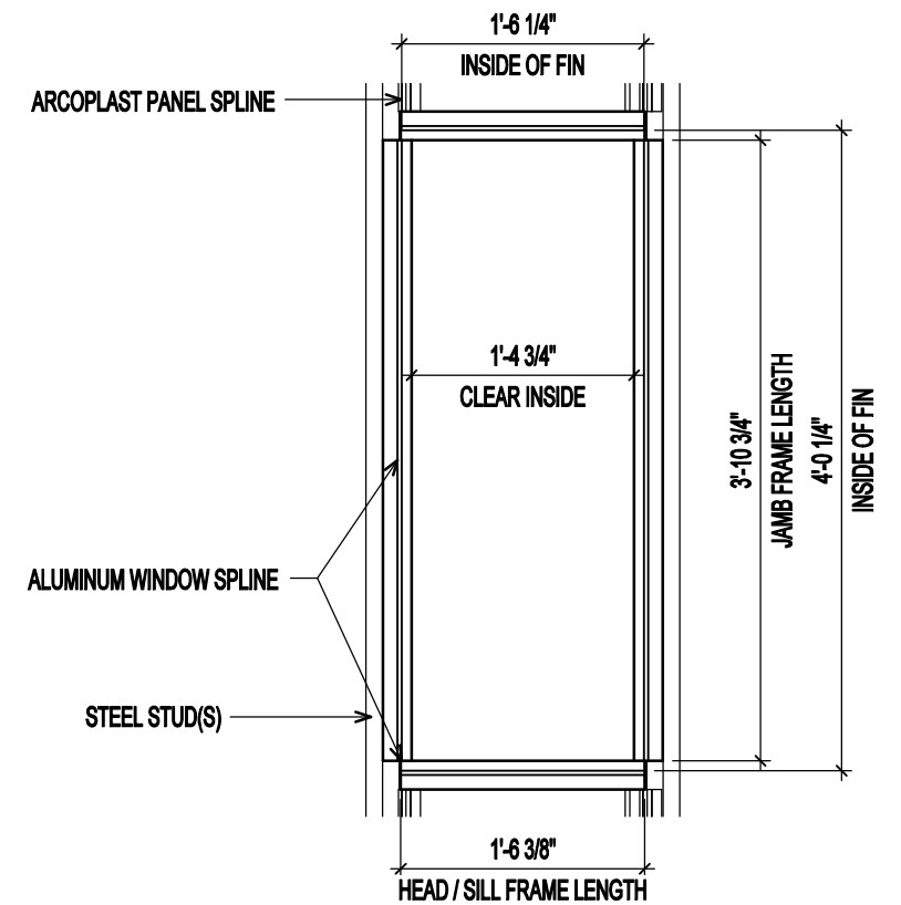
WINDOW ALUMINUM FRAME ELEVATION SCALE: 3/4" = 1'-0" (1:16)
