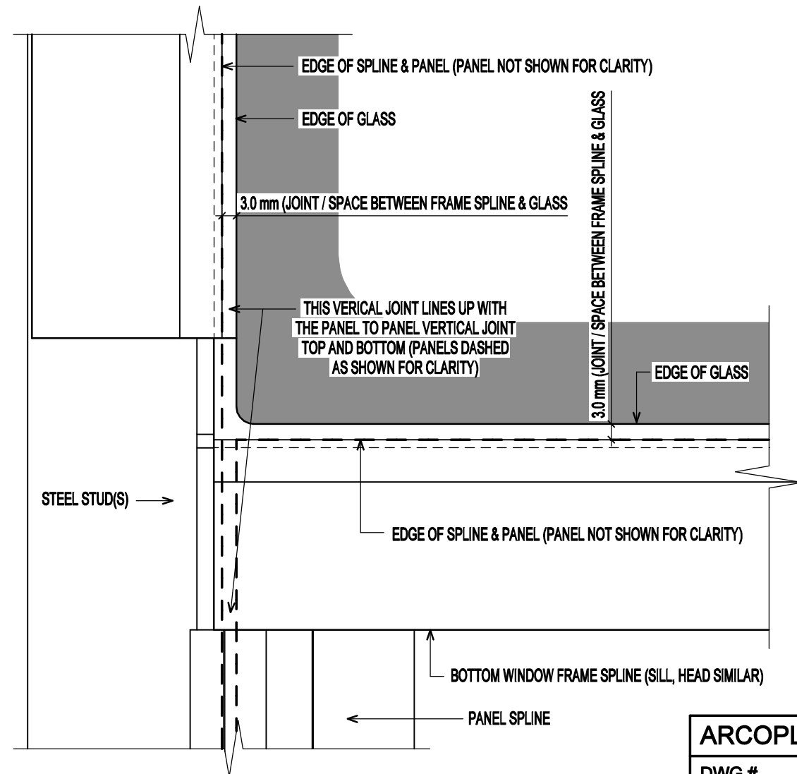
ENLARGED DETAIL AT PANEL / GLASS JOINT SCALE: FULL (1:1)
