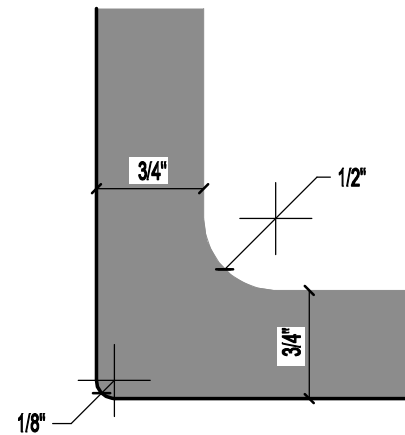
GLASS CORNER DETAIL SCALE: FULL (1:1)
