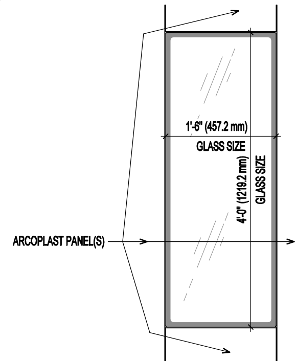
WINDOW ELEVATION
