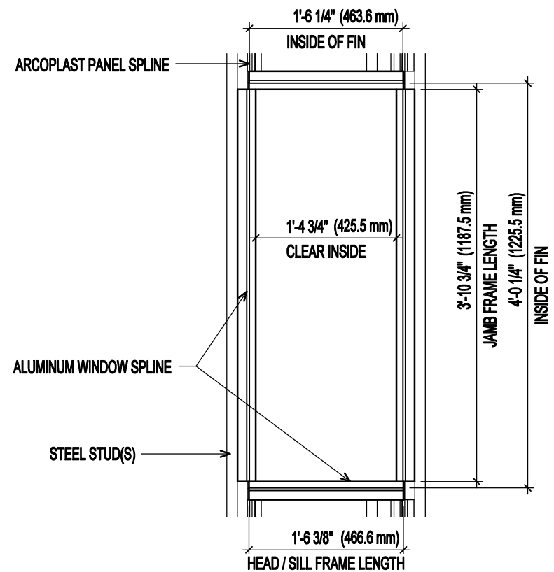
WINDOW ALUMINUM FRAME ELEVATION
