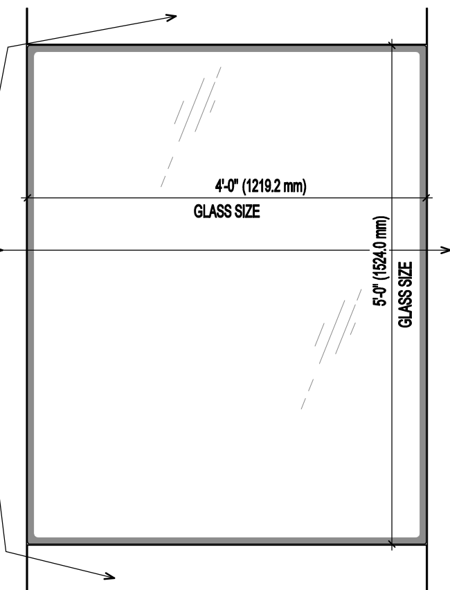
WINDOW ELEVATION
