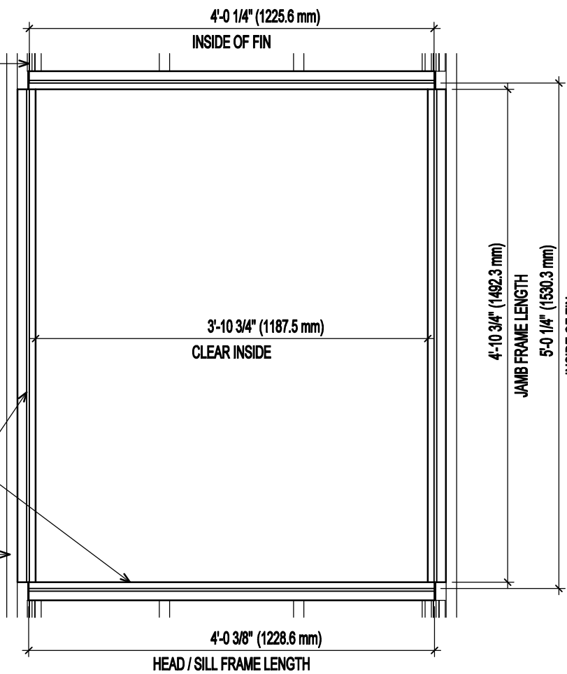
WINDOW ALUMINUM FRAME ELEVATION
