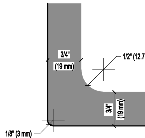
GLASS CORNER DETAIL
