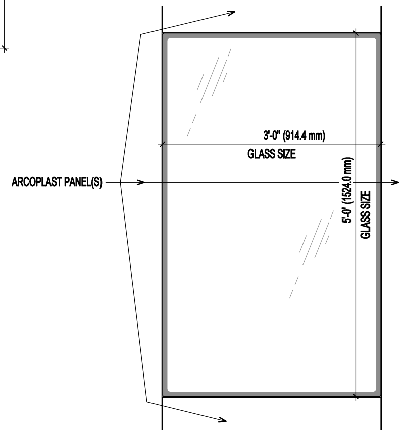
WINDOW ELEVATION
