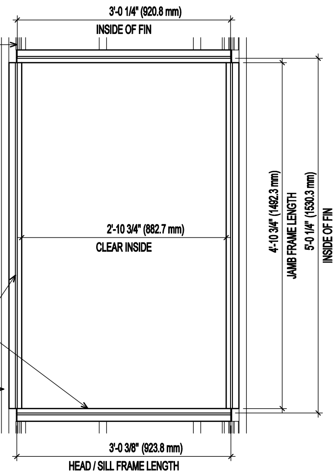
WINDOW ALUMINUM FRAME ELEVATION
