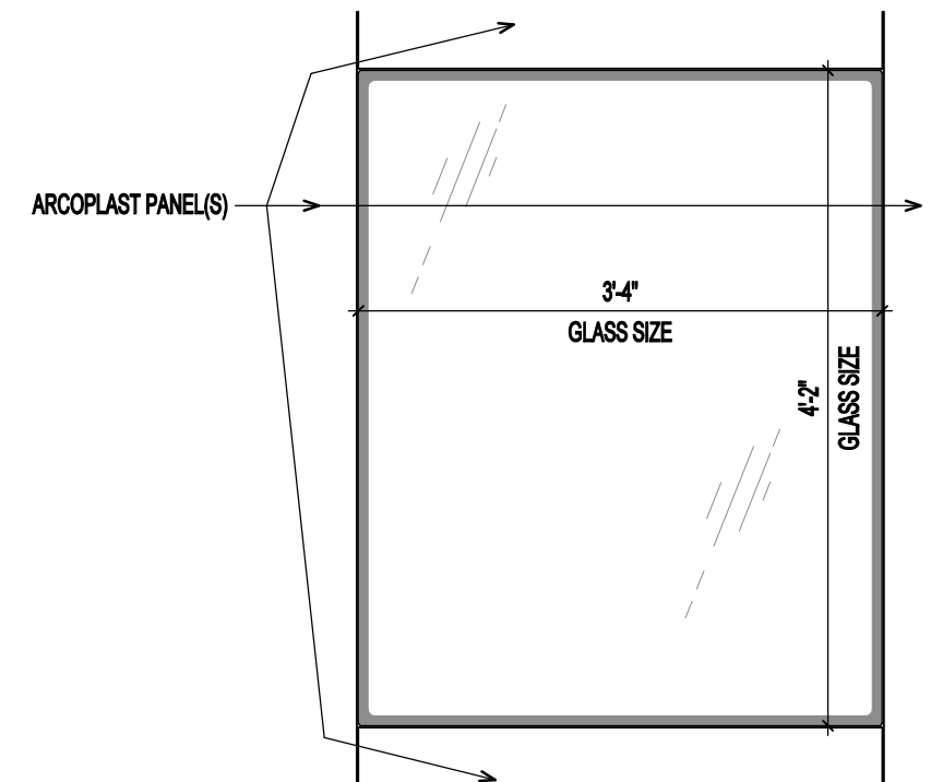
WINDOW ELEVATION
