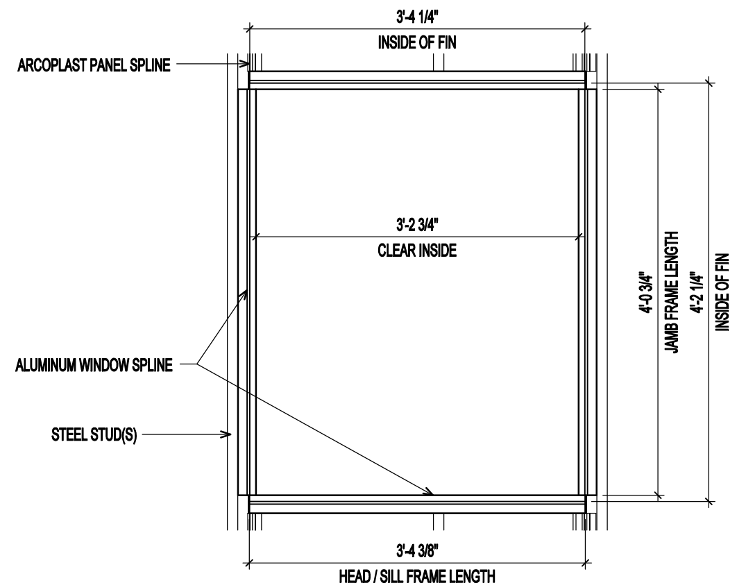
WINDOW ALUMINUM FRAME ELEVATION
