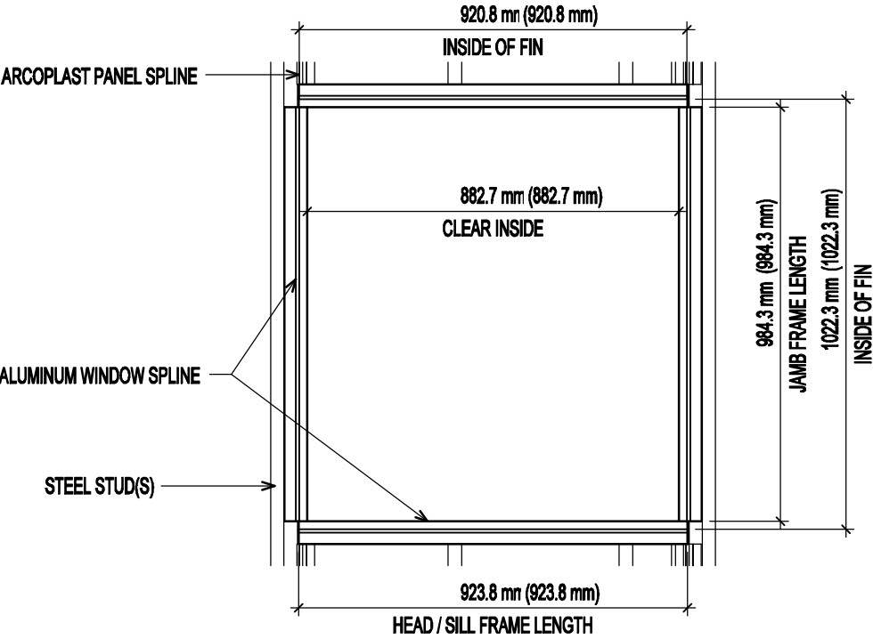
WINDOW ALUMINUM FRAME ELEVATION
