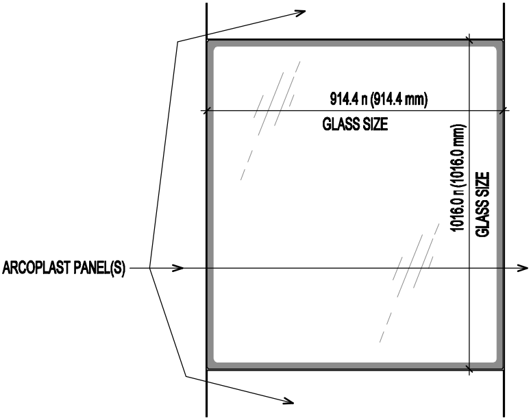
WINDOW ELEVATION
