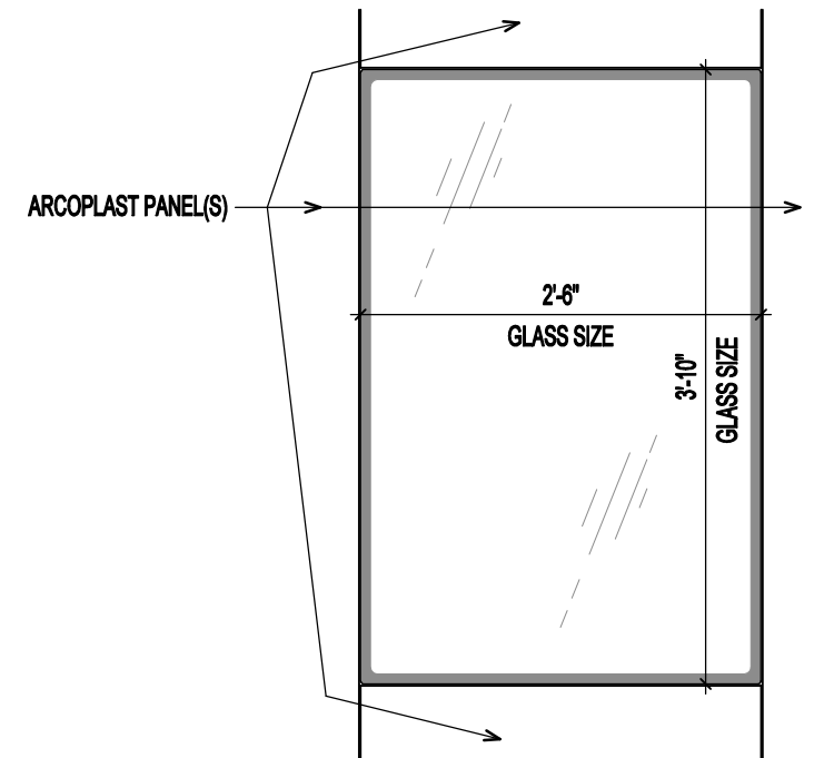
WINDOW ELEVATION SCALE: 3/4" = 1'-0" (1:16)
