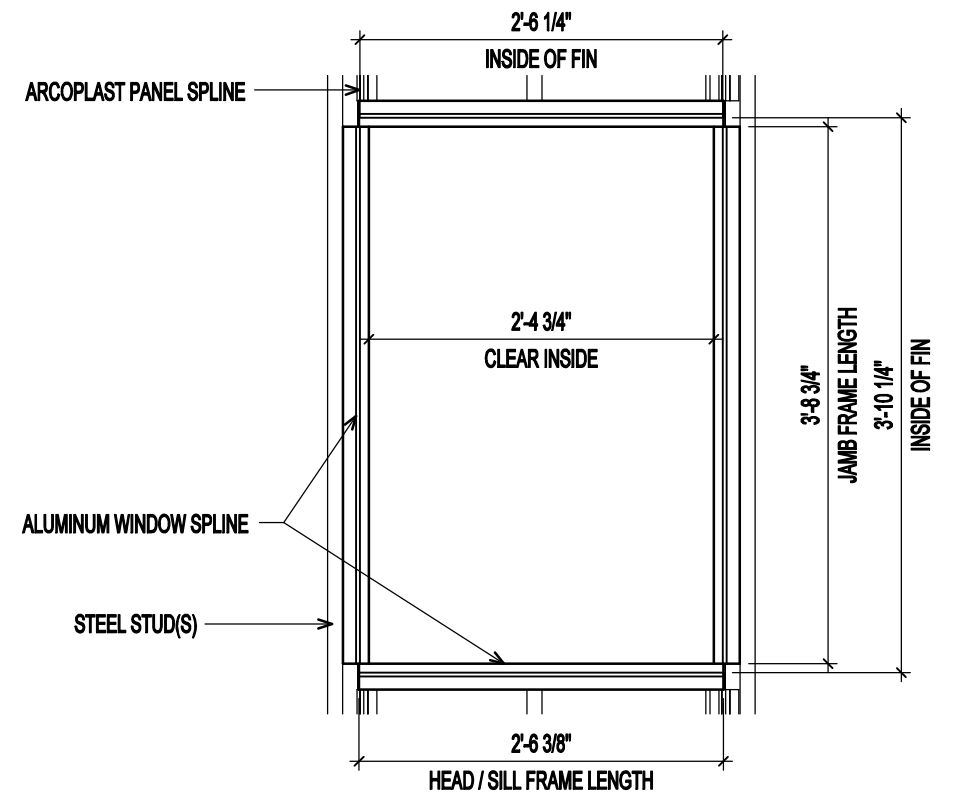
WINDOW ALUMINUM FRAME ELEVATION SCALE: 3/4" = 1'-0" (1:16)
