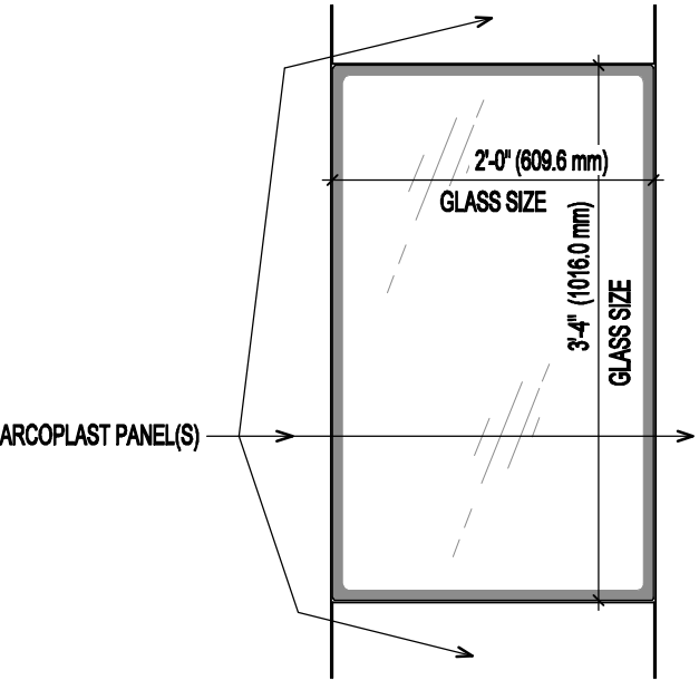
WINDOW ELEVATION
