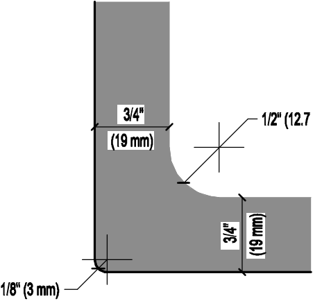
GLASS CORNER DETAIL
