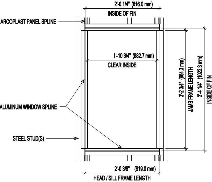
WINDOW ALUMINUM FRAME ELEVATION
